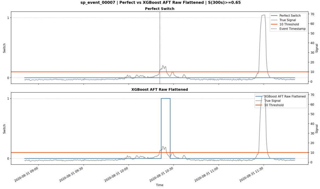
Figure 6.13: False-positive survival switch example for XGBoost-AFT on sp_event_00007 . The model uses S(300\text{s} \mid X_i) \geq 0.65 , the current-signal gate, and common post-processing. Perfect Switch remains zero on the native event; switches outside that segment are displayed as zero for context only.
